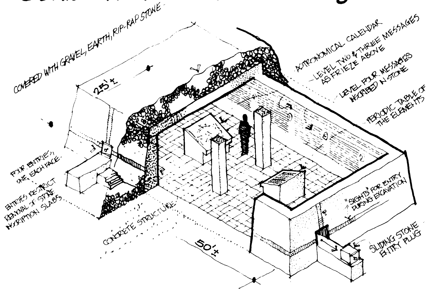
Figure 4.3-17. Buried Room with Level IV Messages (art by Michael Brill).
